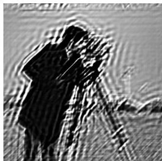
Restored Image
