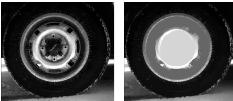
Original Image
