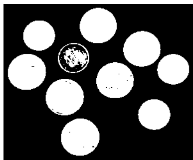
Original Image
