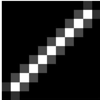
Original PSF
