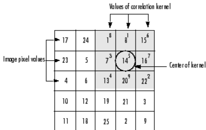
Computing the (2,4) Output of Correlation
