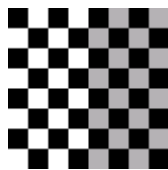
Translated Image
