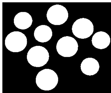
Filled Image
