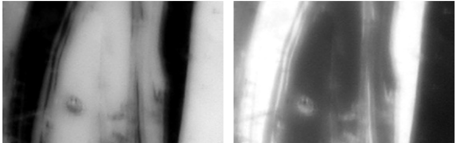
Original Image
